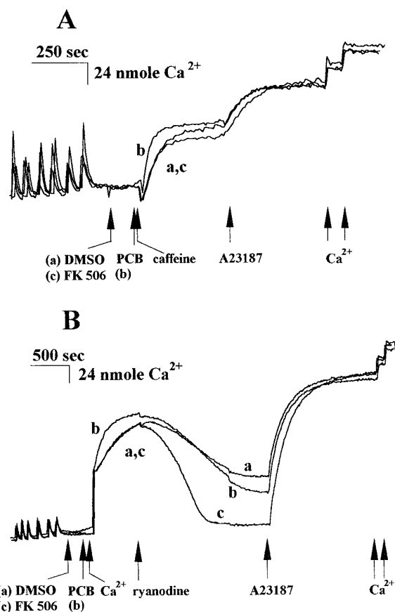
Fig. 3. FK 506 does not affect responses of Ry_1R to caffeine and Ca^{2+} . Vesicles were actively loaded with 144 nmol of Ca^{2+} during the loading phase as described in Experimental Procedures. A , Ca^{2+} release was initiated by the addition of 10 mM caffeine. Trace a , control with 6 \mu l of DMSO followed by 10 mM caffeine. Trace b , 1 \mu M PCB 95 significantly enhanced the rate of caffeine-induced Ca^{2+} release from SR vesicles. Trace c , addition of 50 \mu M FK 506 before 10 mM caffeine did not alter the rate of caffeine-induced Ca^{2+} release. For the experiment shown, the initial rates of caffeine-induced Ca^{2+} release from SR vesicle in the presence of DMSO, PCB 95, and FK 506 were 19.5, 41.0, and 19.0 nmol/mg/sec, respectively. B , CICR was initiated by the addition of a bolus of 84 nmol of Ca^{2+} . Once the Ca^{2+} release was complete, Ca^{2+} reuptake was initiated by the addition of 500 \mu M ryanodine. Trace a , control with 6 \mu l of DMSO followed by the addition of 84 nmol of Ca^{2+} . Trace b , 1 \mu M PCB 95 enhanced the rates of CICR and Ca^{2+} reuptake. Trace c , 50 \mu M FK 506 did not alter the rate of CICR from loaded vesicles but significantly enhanced Ca^{2+} reuptake. For the experiment shown, the initial rates of CICR in the presence of DMSO, PCB 95, and FK 506 were 4.5, 11.0, and 4.0 nmol/mg/sec, respectively. The rates of Ca^{2+} reaccumulation in the presence of DMSO, PCB, and FK 506 were 2.1, 2.4, and 6.4, nmol/mg/sec, respectively. The experiments shown are representative of three replicated measurements with similar results. The rates of caffeine-induced Ca^{2+} release, CICR, and Ca^{2+} reuptake after the addition of ryanodine are summarized in Table 2.
